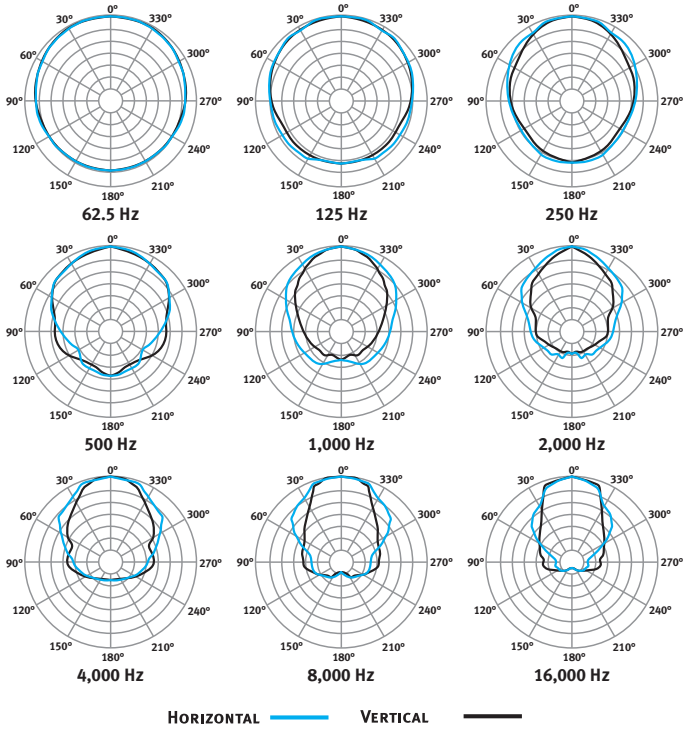
All polar measurements obtained in a free-field environment at 10° increments.
